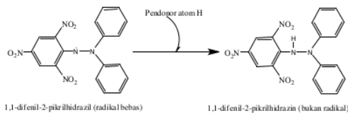
Gambar 3. Reaksi peredaman radikal DPPH
