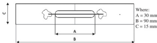
Fig. 3. Single fiber tensile strength specimen.
