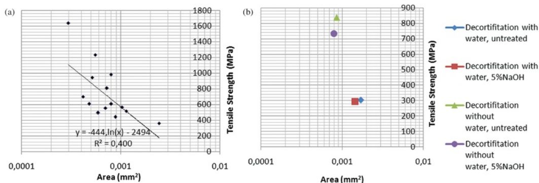
Fig. 5. (a) Correlation area and tensile strength (b) average tensile strength with many types of fiber treatment.
