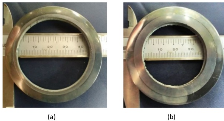
Gambar 4. RSB centrifugal casting (a) 500 rpm, (b) 1000 rpm
