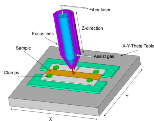
Gambar 2.10 Fiber Laser Microelectronics and Packaging Society
