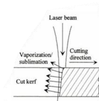
Gambar 2.7 Reactive Cutting (Muhammad, 2012)
