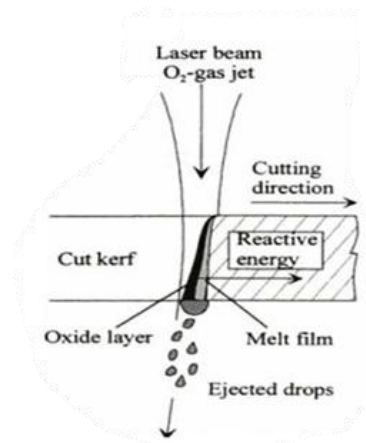
Gambar 2. 7 Ilustrasi Vaporization Cutting
