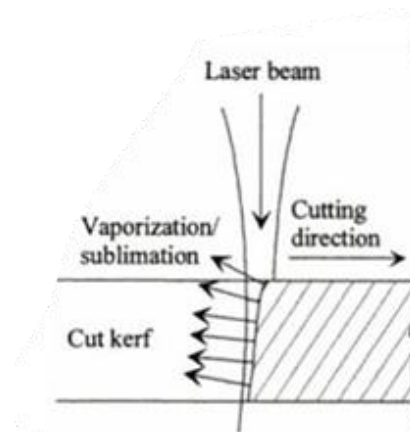
Gambar 2. 8 Reactive Cutting
