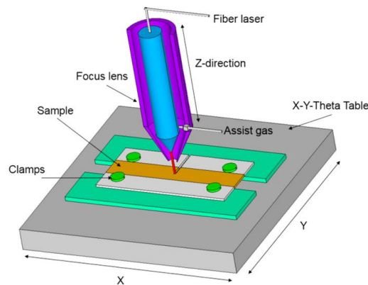
Gambar 2. 11 Fiber Laser
