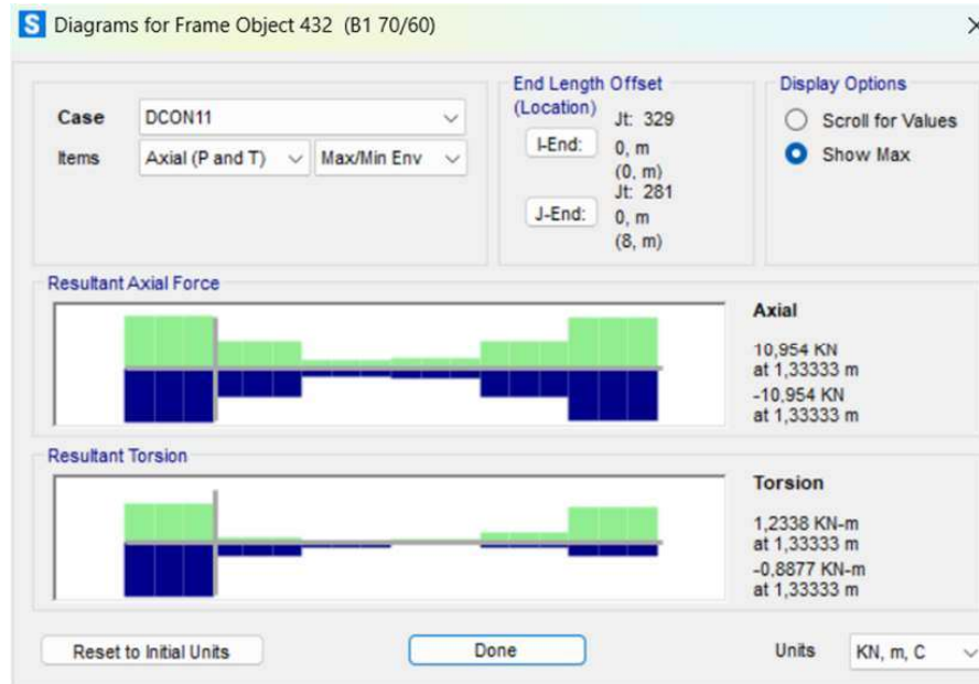
Gambar 4. 7 Output Gaya Aksial Balok B1
