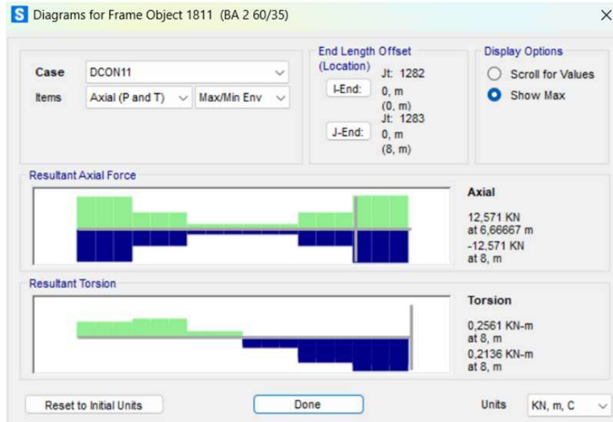
Gambar 4. 43 Output Gaya Aksial Balok BA2
