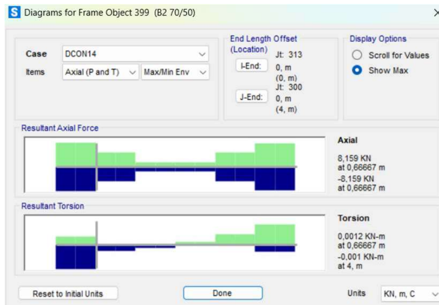
Gambar 4. 16 Output Gaya Aksial Balok B2
