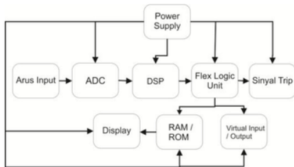
Gambar 3. Blok Diagram IED Relai Proteksi
