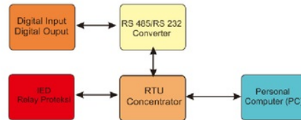
Gambar 2. Blok Diagram
