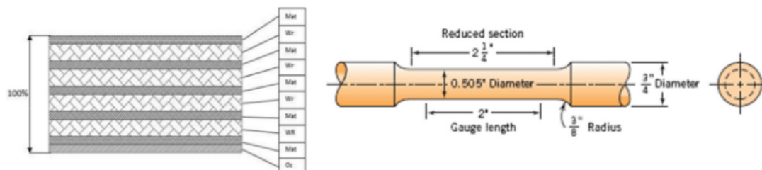
Fig. 1. Glass fiber layer and dimension and size of the specimen
