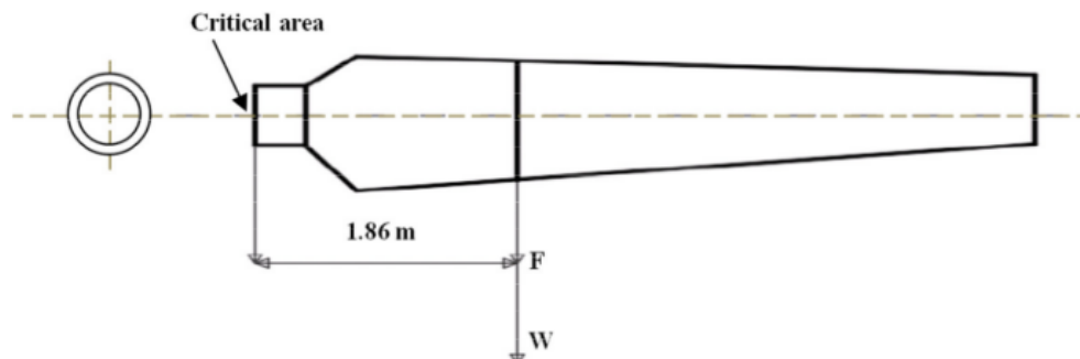
Fig. 2. Load of blade critical area
