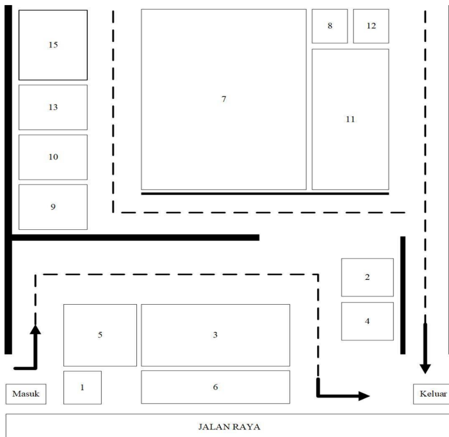
Gambar 2.5 Layout Pabrik
