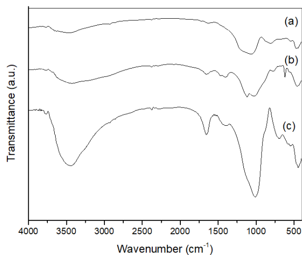
Fig. 2. FTIR spectra of metakaolin (a), biomass ash (b), and geopolymer (c).
