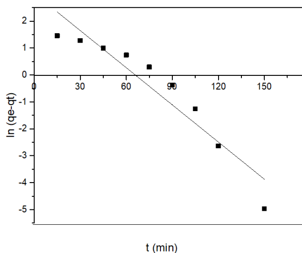
Fig. 9. Linear plot of pseudo-first order kinetics model on Cu(II) ions adsorption by geopolymer.
