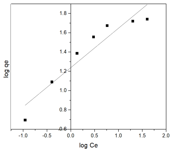
Fig. 12. Linear plot of Freundlich isotherm model on Cu(II) ions adsorption by geopolymer.
