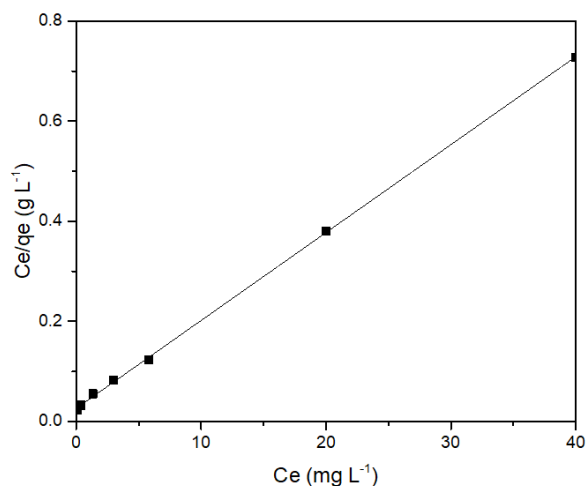
Fig. 11. Linear plot of Langmuir isotherm model on Cu(II) ions adsorption by geopolymer.
