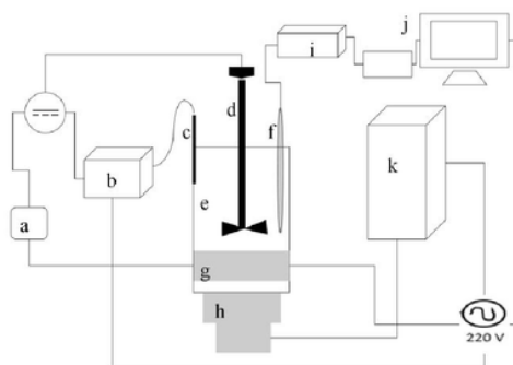
Figure 1. Experimental set up of extraction system using UAE. a: relay, b: thermocontroller, c: thermocouple, d: mixer, e: tank, f: LM35, g: heater, h: transducers, i: microcontroller, j: mini PC, k: ultrasound power supply.
