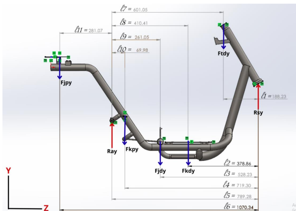
Gambar 2. 13 Free body diagram
