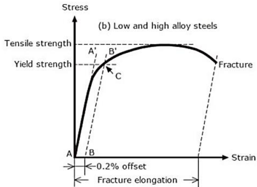
Gambar 2. 7 Grafik low and high alloy steels
