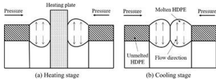
Gambar 2. 2 Butt fusion
