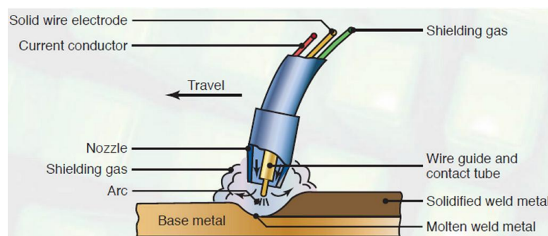
Gambar 2. 8 Proses pengelasan GTAW Sumber : (SLV Metropolitan Indonesia, 2019)
