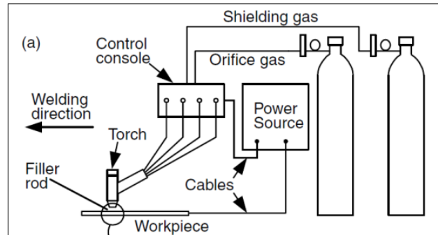
Gambar 2. 10 Proses plasma ARC welding Sumber : (Waisya, 2011)
