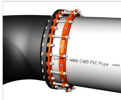
Gambar 2. 5 Mechanical joint
