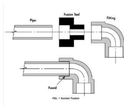
Gambar 2. 3 Socket fusion
