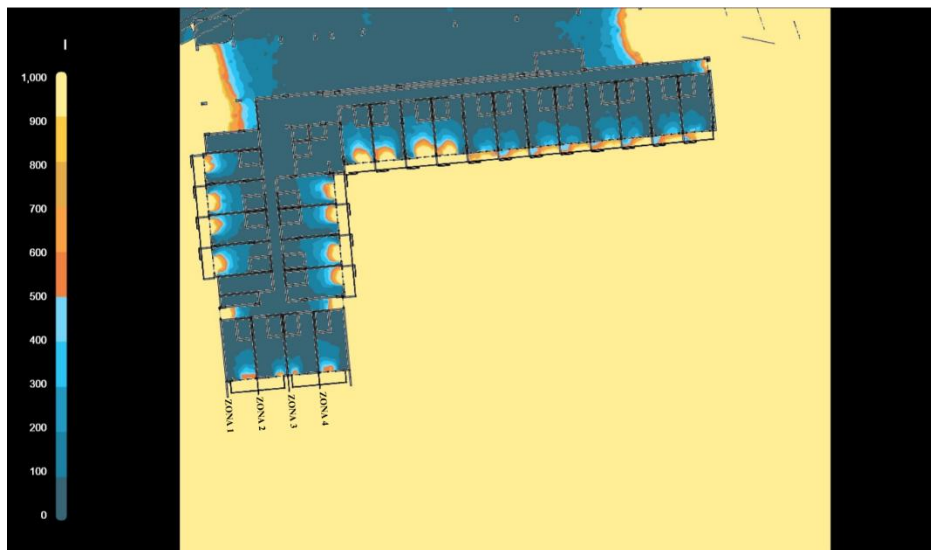
Gambar IV.126 Hasil Simulasi Fasad Overhang Sunshading Lantai 4 Jam 12.00
