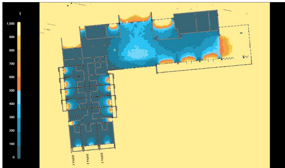
Gambar IV.130 Hasil Simulasi Fasad Overhang Sunshading Lantai 5 Jam 15.00
