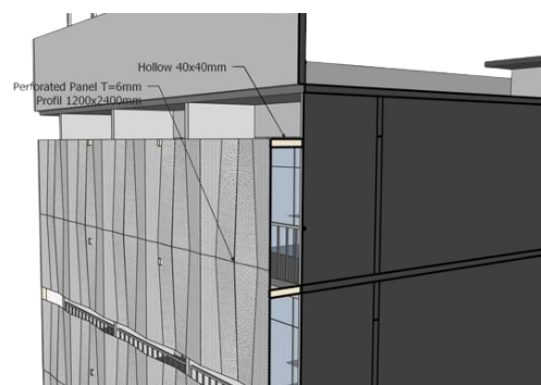
Gambar IV.73 Blow Up Hasil Redesain Fasad Perforated Panel
