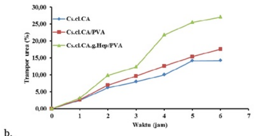
Gambar 4. Persentase transport kreatinin (a) dan (b) urea.
