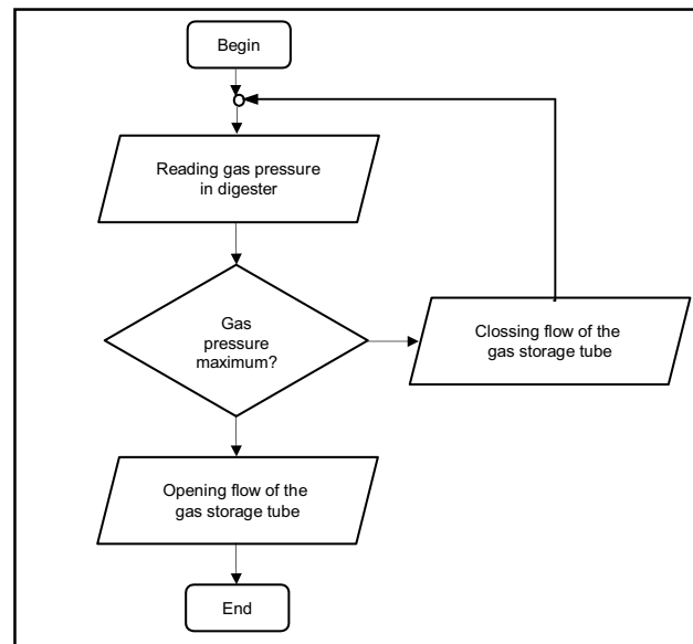
Figure 6. The main algorithm
