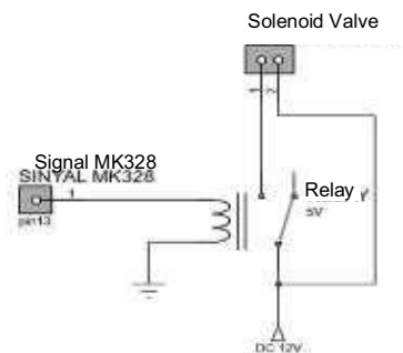
Figure 5. Solenoid valve driver circuit
