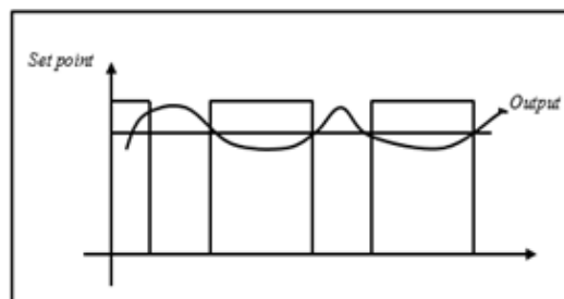
Figure 1. Illustration of on-off control signal ( www.reocities.com/al_dodi/kp3.pdf )
