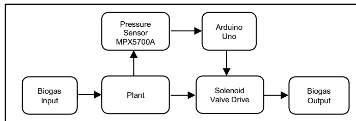
Figure 4. The block diagram of control system
