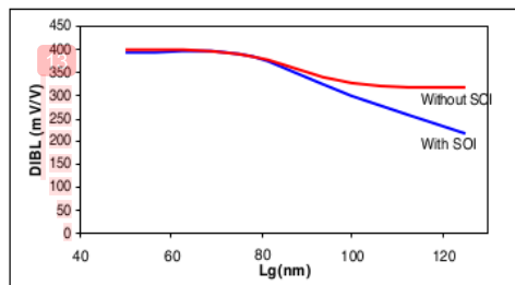
Fig. 5. DIBL Graph
