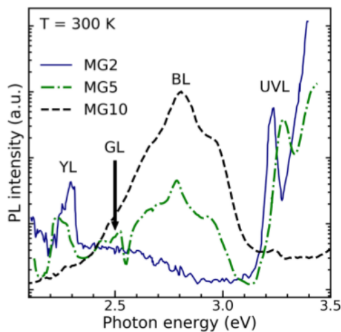
FIG. 2. PL spectra of plasma-assisted MOCVD-grown Mg-doped GaN with \text{Cp}_2\text{Mg} flow rates of 2% (MG2), 5% (MG5), and 10% (MG10) of the total flow rate.
