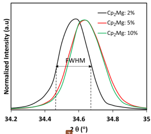
FIG. 6. Normalized XRD spectra of Mg-doped GaN with various Cp_2Mg flow rates (2%, 5%, and 10% of the total flow rate for samples MG2, MG5, and MG10, respectively). The diffraction peaks of samples MG5 and MG10 are shifted to a higher angle, indicating an increase in the lattice constant.
