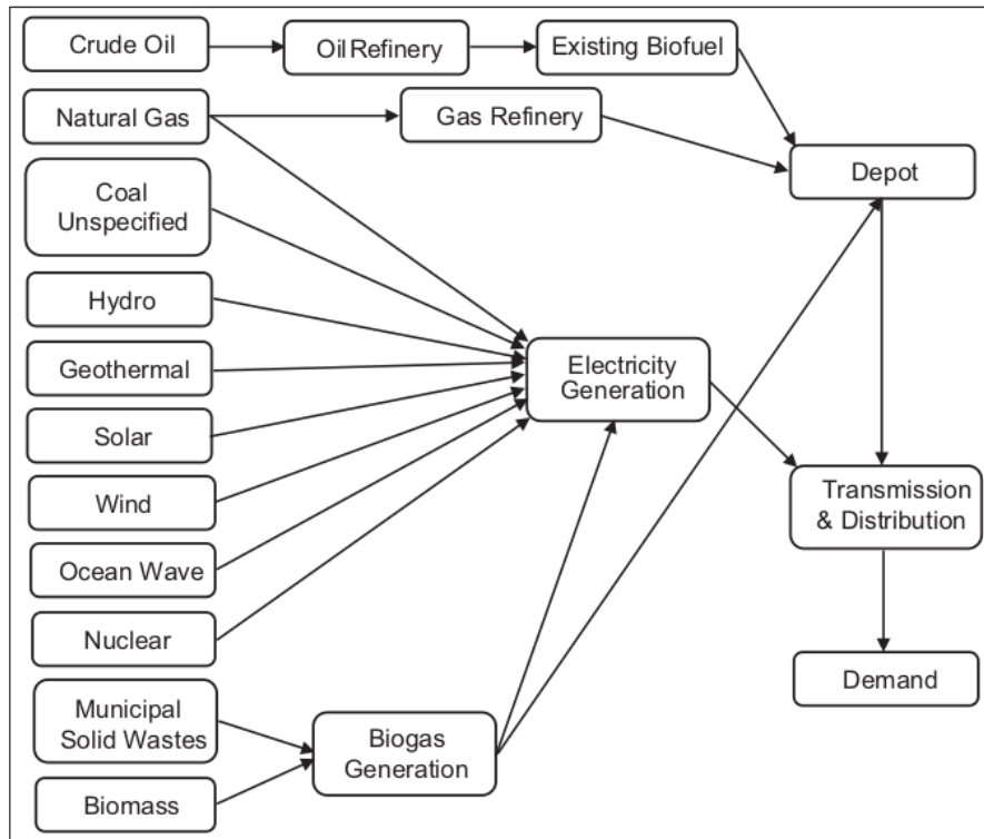
Figure 1: Reference energy system
