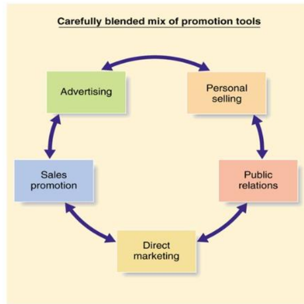
Gambar 5 IMC Tools
