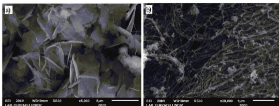
Figure 2: Test results of ZnO and MWCNT magnification 5000X with a) ZnO hydrothermal 160°C, and b) MWCNT.
