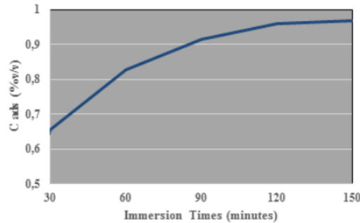
Fig 2. The Relationship of The Immersion Times of Mangosteen Peel To Adsorbed Concentration of Dye on TiO 2
