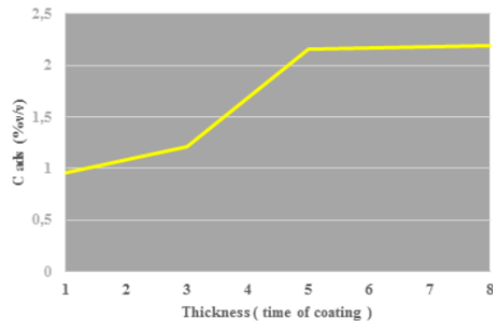
Fig 3. The Relationship of The Electrode Thickness To Adsorbed Concentration of Dye on TiO 2
