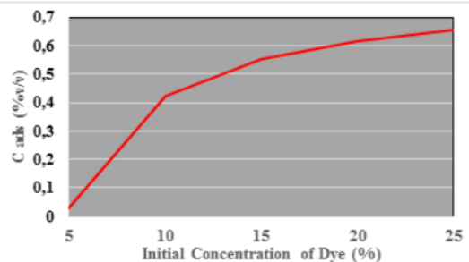
Fig 1. The Relationship of The Initial Extract Concentration of Mangosteen Peel To Adsorbed Concentration of Dye on \text{TiO}_2
