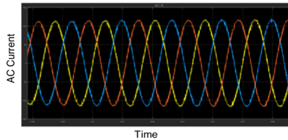
Figure 9. AC Current Wave of Three Phase Inverter Output T = 1273 K
