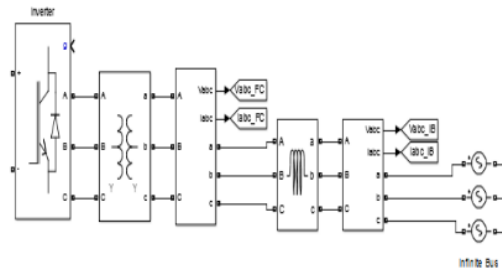
Figure 3. The series Inverters connected to the Grid
