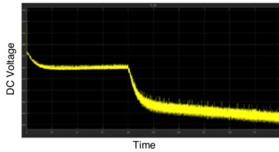
Figure 10. DC Voltage Graph SOFC with 350 cells
