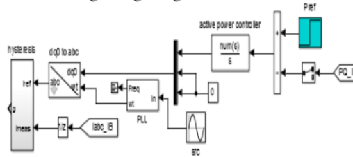
Figure 2. Grid-side Controller Series.
