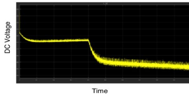
Figure 7. Graph of DC Voltage SOFC T = 1273 K
