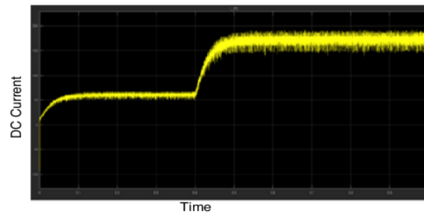
Figure 8. DC Current Graph SOFC T = 1273 K
