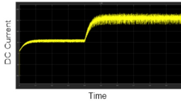
Figure 5. DC current Graph SOFC T = 873 K
