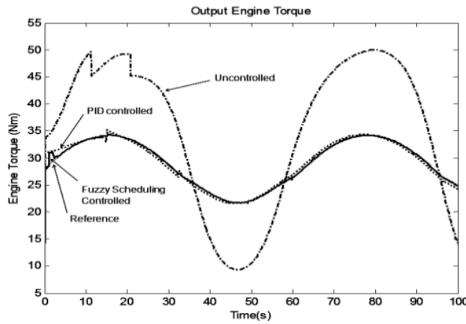
Figure 9. Simulation result for engine torque output with sinusoidal throttle input
