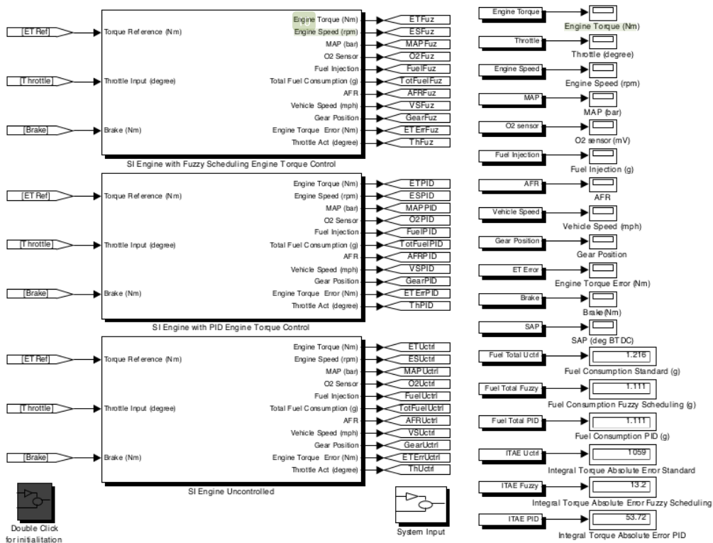
Figure 5. Simulation main model using Matlab Simulink Toolbox
