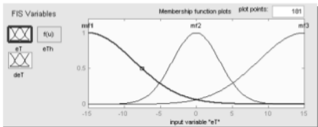
Figure 2. Membership functions of engine torque input error
