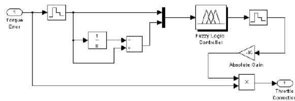
Figure 6. Fuzzy gain scheduling simulation sub-model using Matlab Simulink Toolbox
