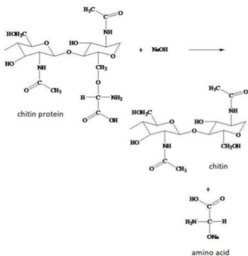
Figure 1. Deproteinization reaction
