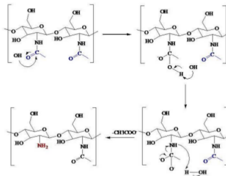
Figure 2. Deacetylation reaction
