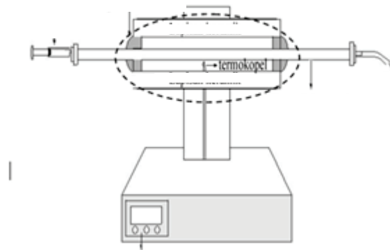
FIGURE 1. Spray Pyrolysis System used for CNT Production
