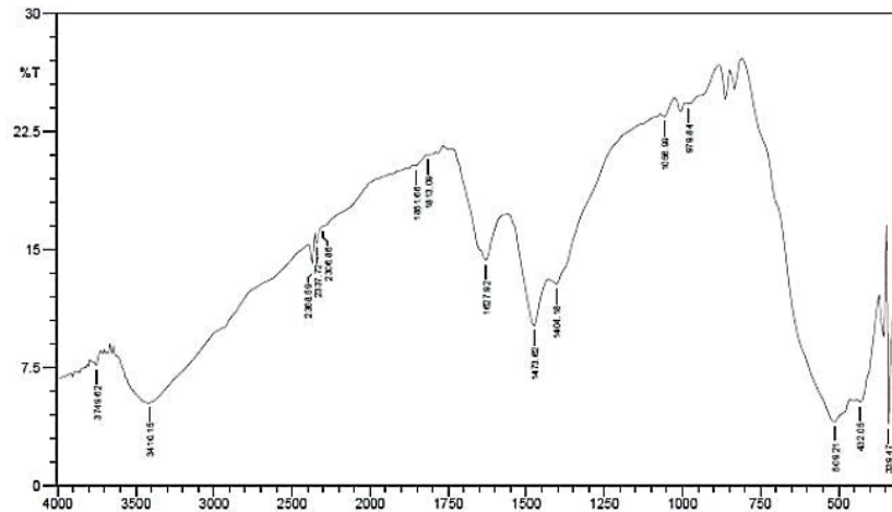
FIGURE 4. IR Spectra of MnO 2
