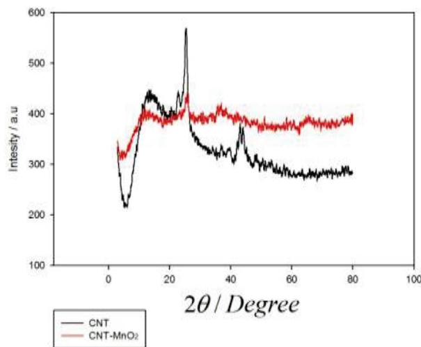
FIGURE 9. XRD Diffractogram Analysis of CNT/MnO 2
