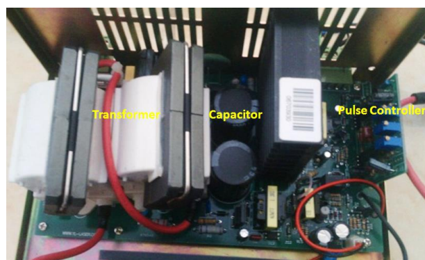
Fig. 2. Electric power supply electrospinning machine.
