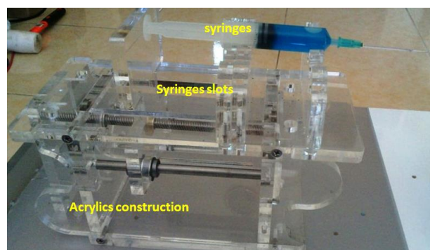
Fig. 3. Syringe electrospinning pump.
