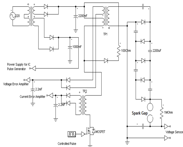
Fig. 1. High Voltage electronic circuit for electrospinning device.
