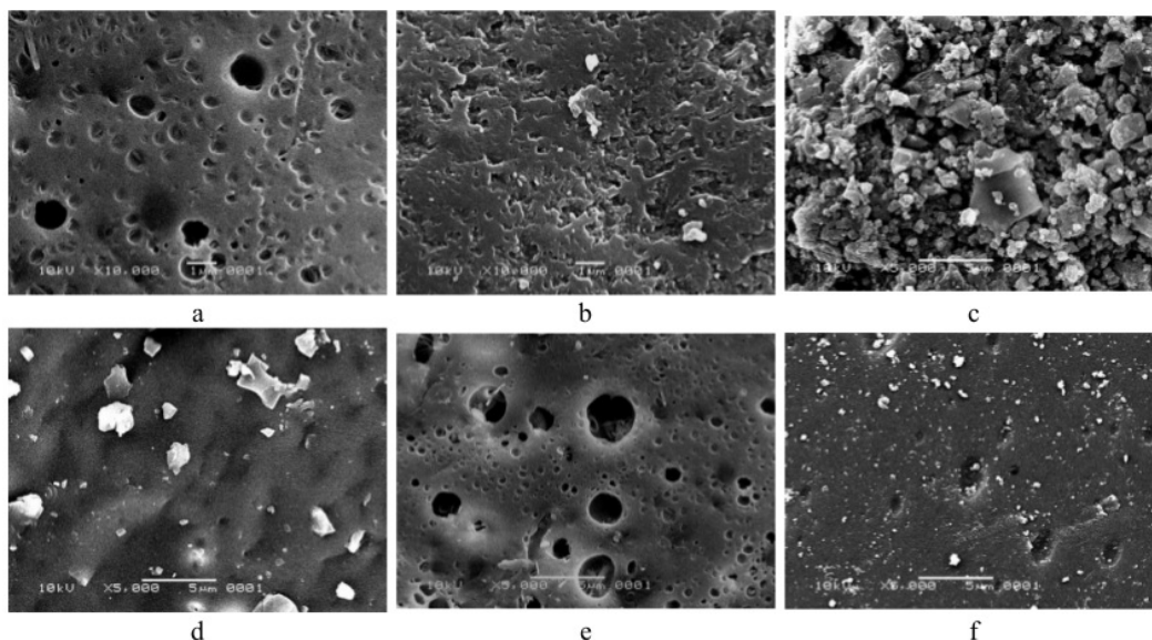
Figure 2. SEM images of (a) EOA-Cr-EGDMA, (b) EOA-EGDMA, (c) Eug-Cd-DVB 10%, (d) Eug-DVB 10%, (e) Poly-Cr-DVB, (f) Poly-DVB
