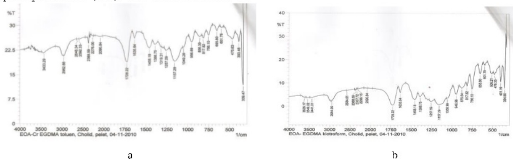
Figure 1. FTIR spectra of (a) EOA-Cr-EGDMA and (b) EOA-EGDMA
