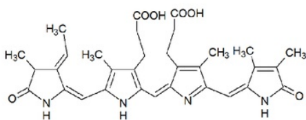
Figure 1. Phycocyanin chemical structure.
