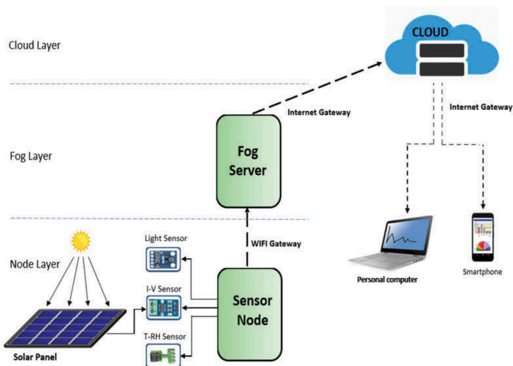
Figure 3. Diagram of a fog network communication system.
