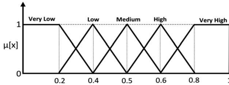
Figure 2. Fuzzy membership function according to sensor readings.
