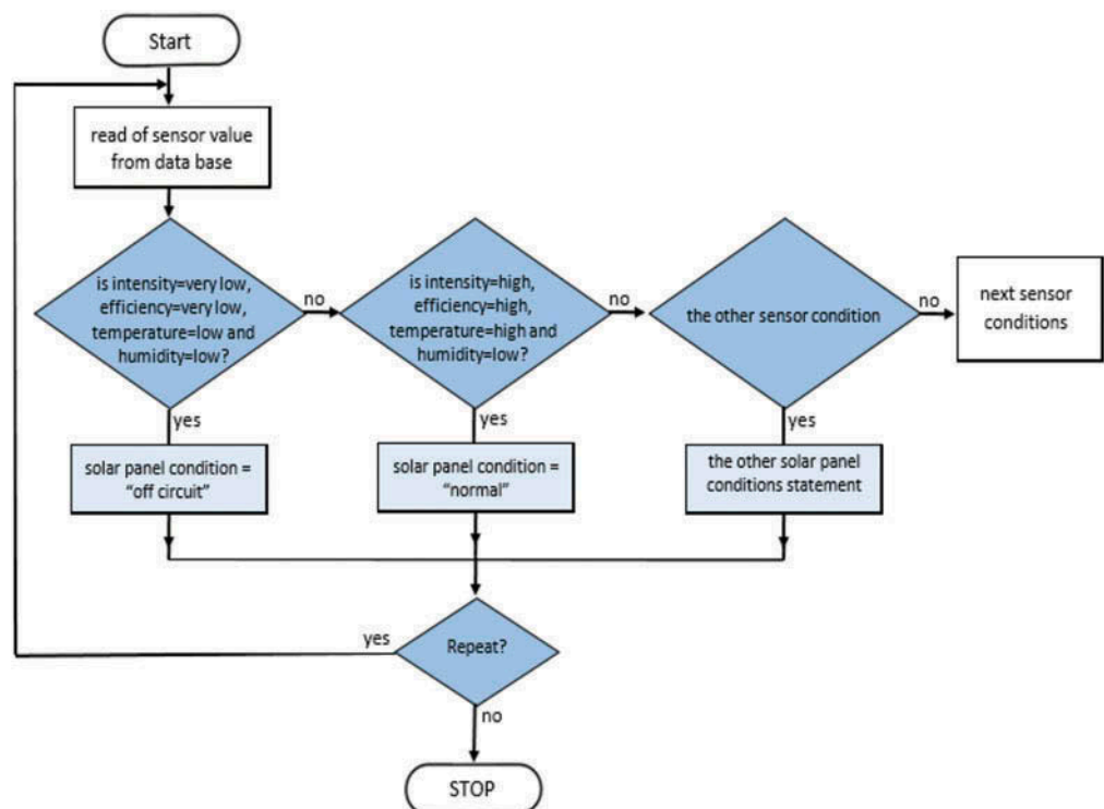
Figure 7. Diagram of rule-based system flow.
