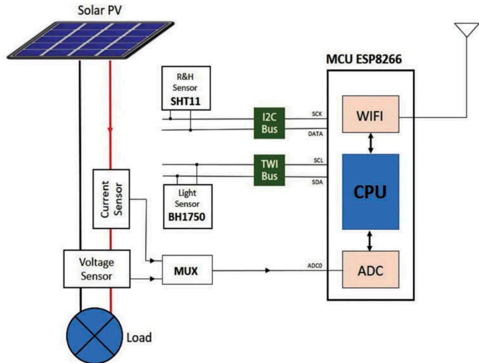
Figure 4. Diagram of sensor communication system circuit with SoC Wi-Fi microcontroller ESP8266.
