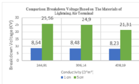
Fig. 4. Comparison breakdown voltage
