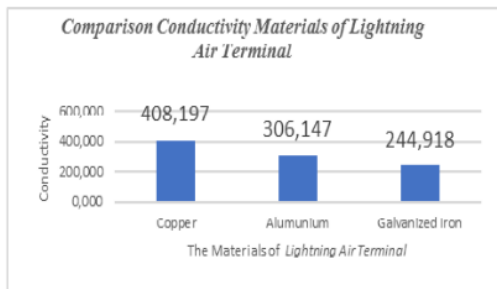
Fig. 5. Comparison conductivity of materials
