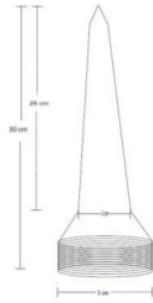
Fig. 1. Dimension of Lightning air terminal
