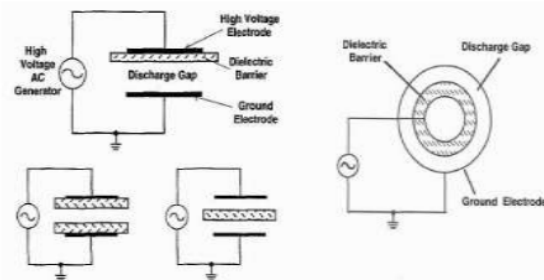
Fig. 1 Common dielectric-barrier discharge configurations
