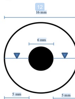
Fig 2. Geometry Plasma DBD Reactor
