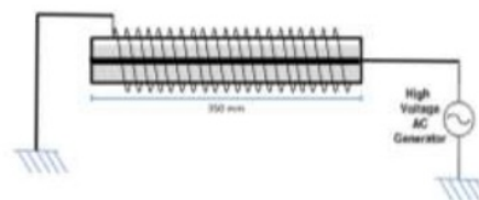
Fig 4. Test Circuit for Generating DBD Plasma
