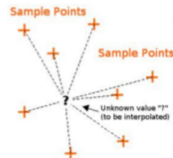
Gambar 1. Inverse Distan Weighted
