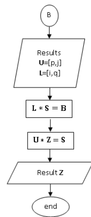
Figure 2. Flowchart Crout decomposition
