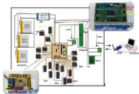
Gambar 3. Assembly hardware elektronik hexapod robot
