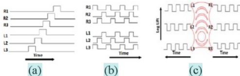
Gambar 8. Skema one wave (a) two wave , dan tripod (c) [22]
