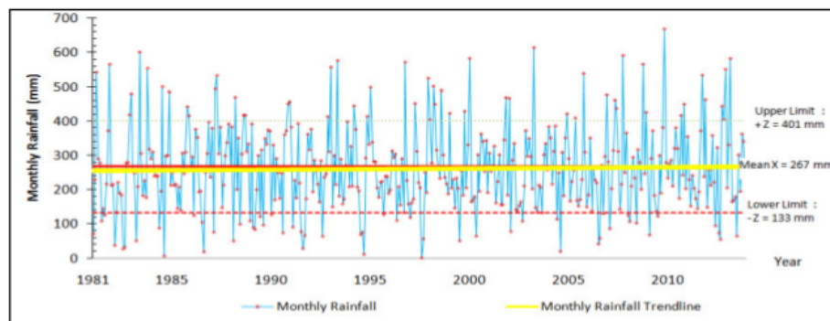
Fig. 3. Monthly rainfall and trendline monthly rainfall 1981-2013.
