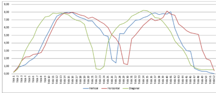
Figure 6 Wind velocity distribution curve before through flow straightener for measurement in vertical, horizontal, and diagonal position
