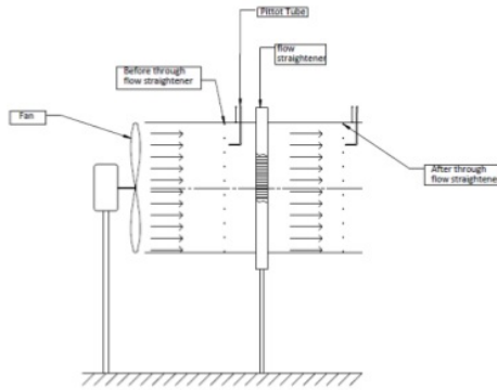
Figure 3 Test facility set up
