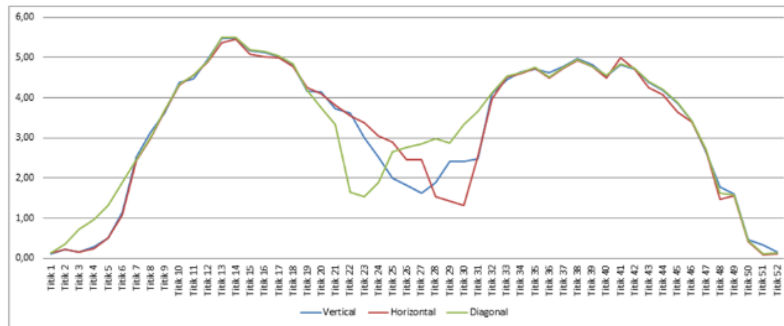
Figure 7 Wind velocity distribution curve after through flow straightener for measurement at vertical, horizontal, and diagonal position
