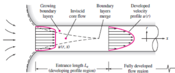
Figure 1 Flow condition in pipe con [6]
