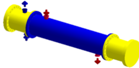
Gambar 4. Shell and tube layout
