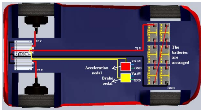
Fig. 5. Wiring diagram for component of the electric car
