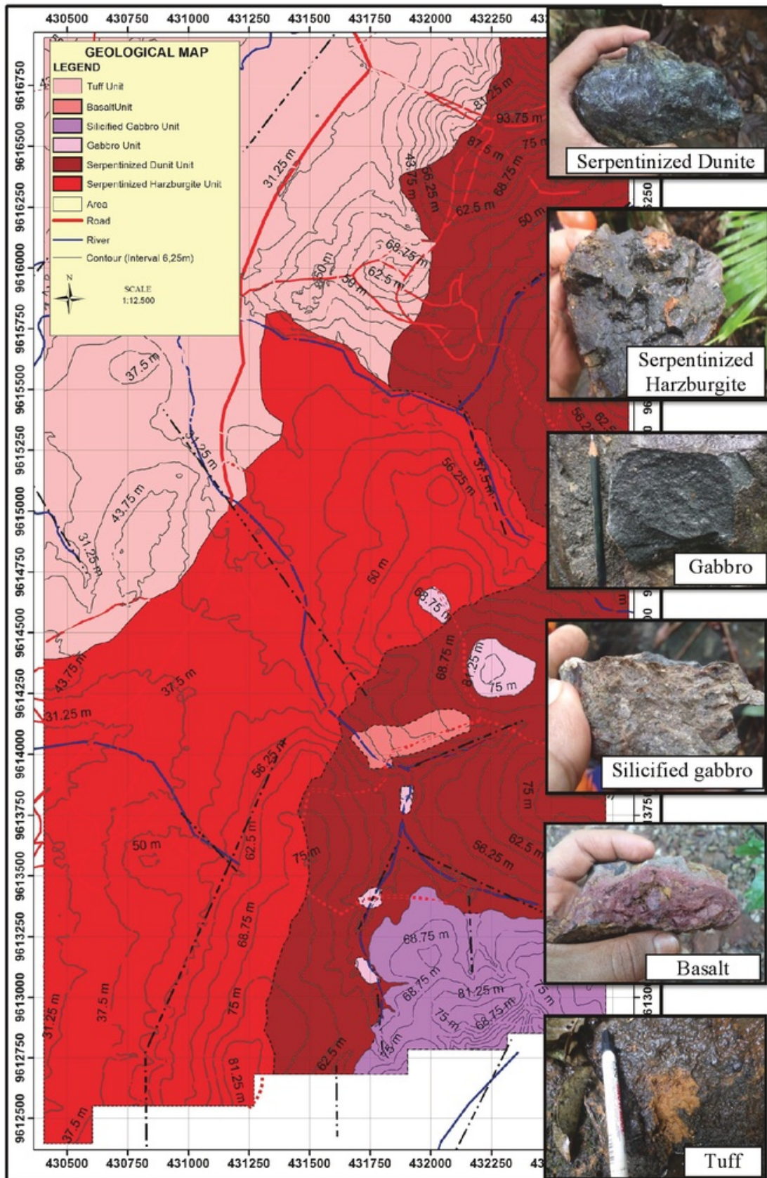
Fig. 1. Geological map and rock samples of research areas.
