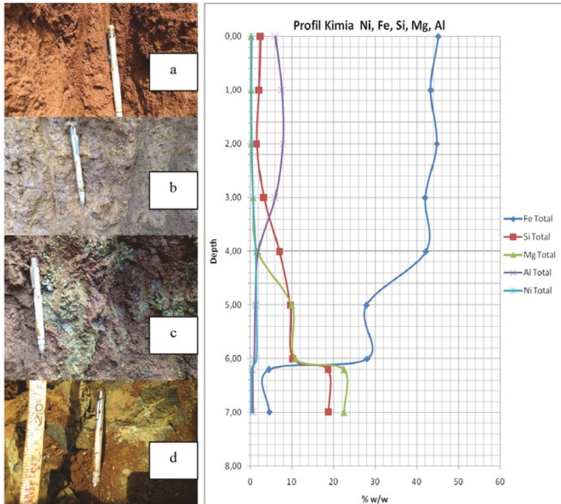
Fig. 2. Laterite and chemical profile.
