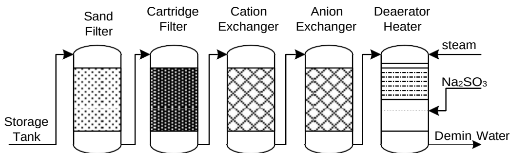
Gambar 4. 2. Proses demineralisasi air.
