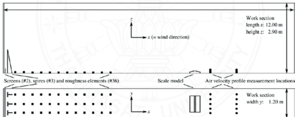
Fig 1. Longitudinal cross section and top view of the wind tunnel work section, with x = 0 m at the far left and the scale model placed at x = 7.67 m. The filled circles denote the positions where air velocity profiles were registered at x = 8.51 m and x = 9.59 m.
