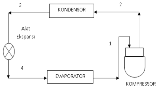
Gambar 2. 1 Siklus refrigasi standar
