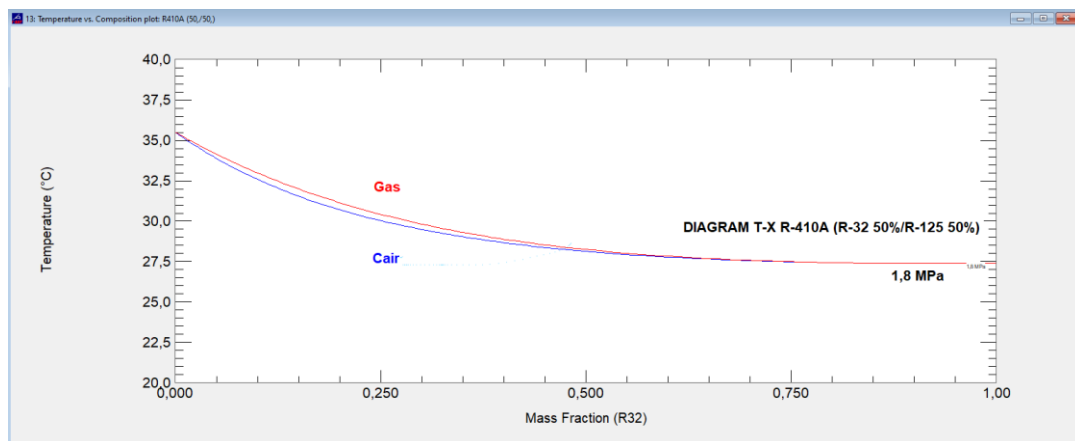
Gambar 2. 10 Diagram T-X R-410A
