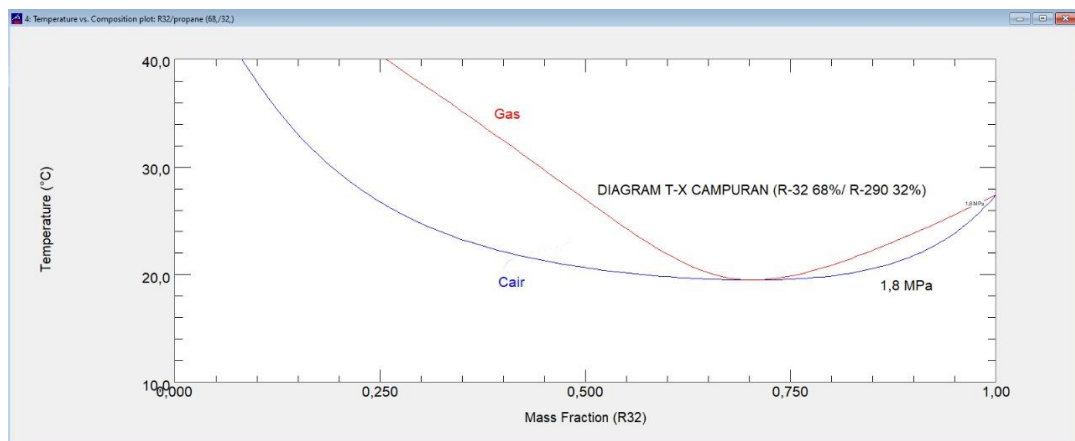
Gambar 2. 11 Diagram T-X R-32/R-290
