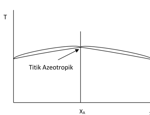
Gambar 2. 9 Diagram T-X Campuran Azeotropic Sumber: (Widodo, 2024)
