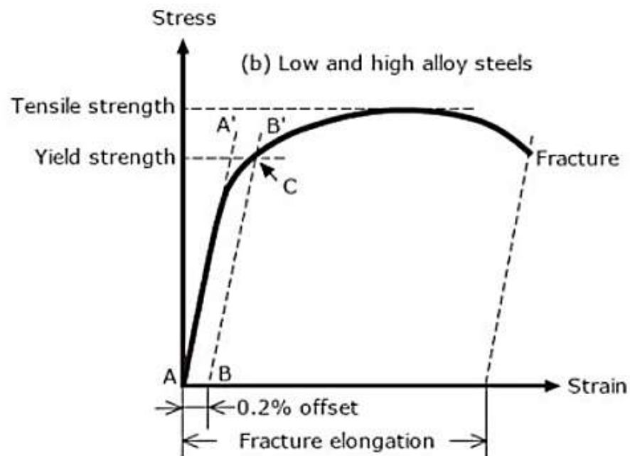
Gambar 2. 6 Grafik low and high alloy steels Sumber : Callister, W. D., & Rethwisch, D. G., 2020
