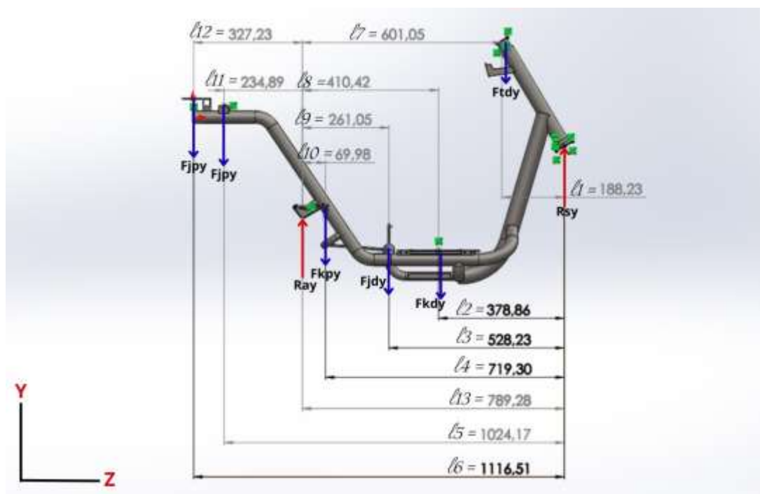
Gambar 2. 12 Free body diagram
