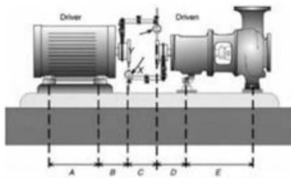
Gambar 2. 13 Shaft alignment metode reverse dial
