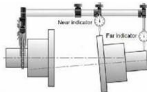
Gambar 2. 11 Double radial
