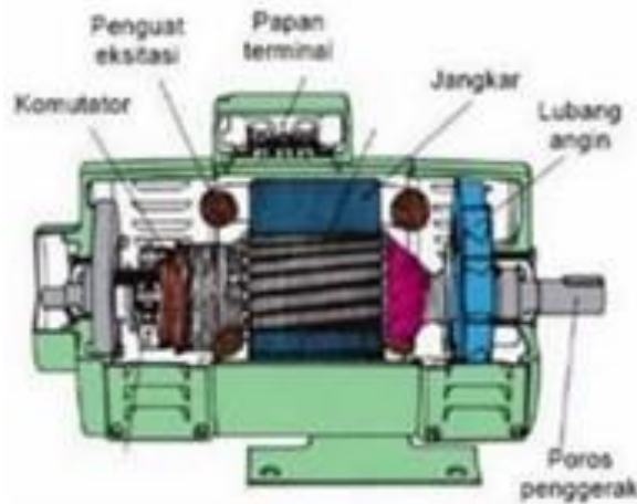
Gambar 2. 2 Generator DC
