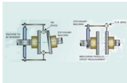
Gambar 2. 8 Face and Rim
