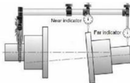
Gambar 2. 11 Double radial
