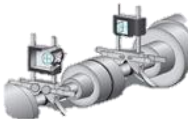
Gambar 2. 16 Shaft alignment metode laser
