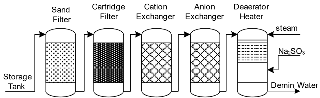
Gambar 4. 2. Proses demineralisasi air.
