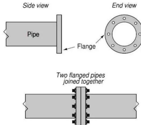
Gambar 2. 6 Flange joint
