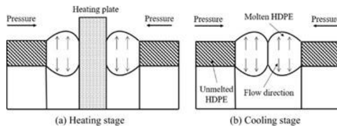
Gambar 2. 2 Butt fusion
