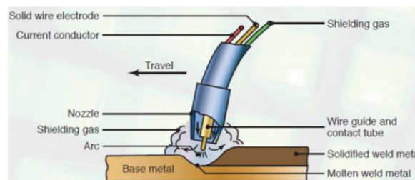
Gambar 2. 8 Proses pengelasan GTAW Sumber : (SLV Metropolitan Indonesia, 2019)
