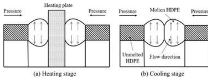
Gambar 2. 12 Proses pengelasan manual butt fusion
