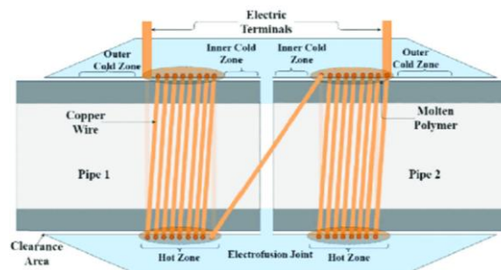
Gambar 2. 4 Electrofusion
