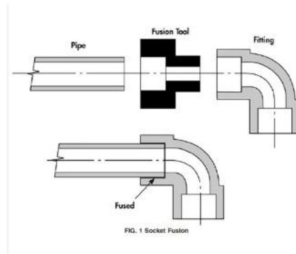
Gambar 2. 3 Socket fusion
