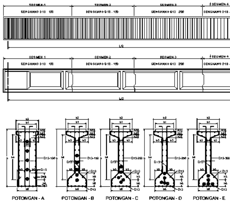
Gambar 4. 48 Detail Senggang
