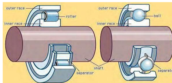
Gambar 2.15 Bantalan ( bearing )
